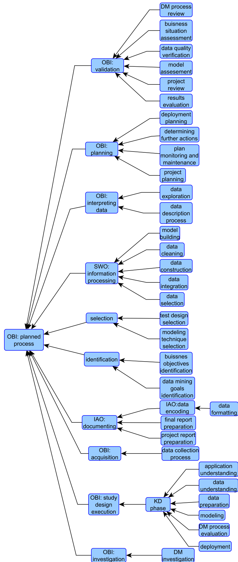
Figure 7.3: Upper level processual classes in OntoDM-KDD ontology.
