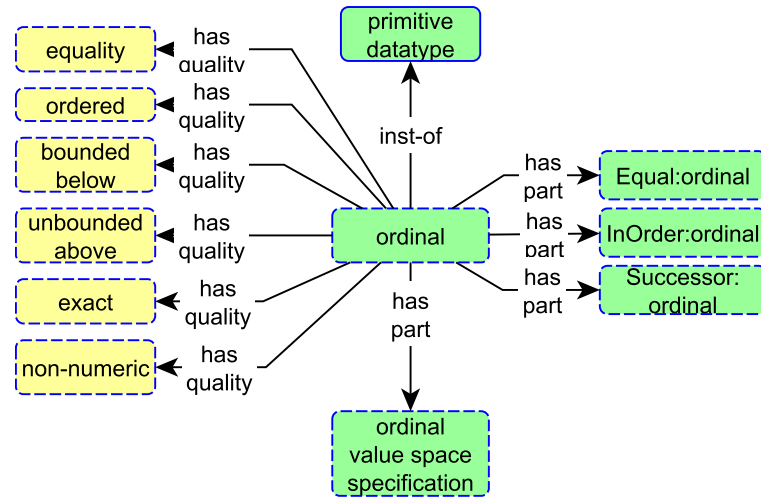
Figure 5.8: The ordinal datatype class in OntoDT.
