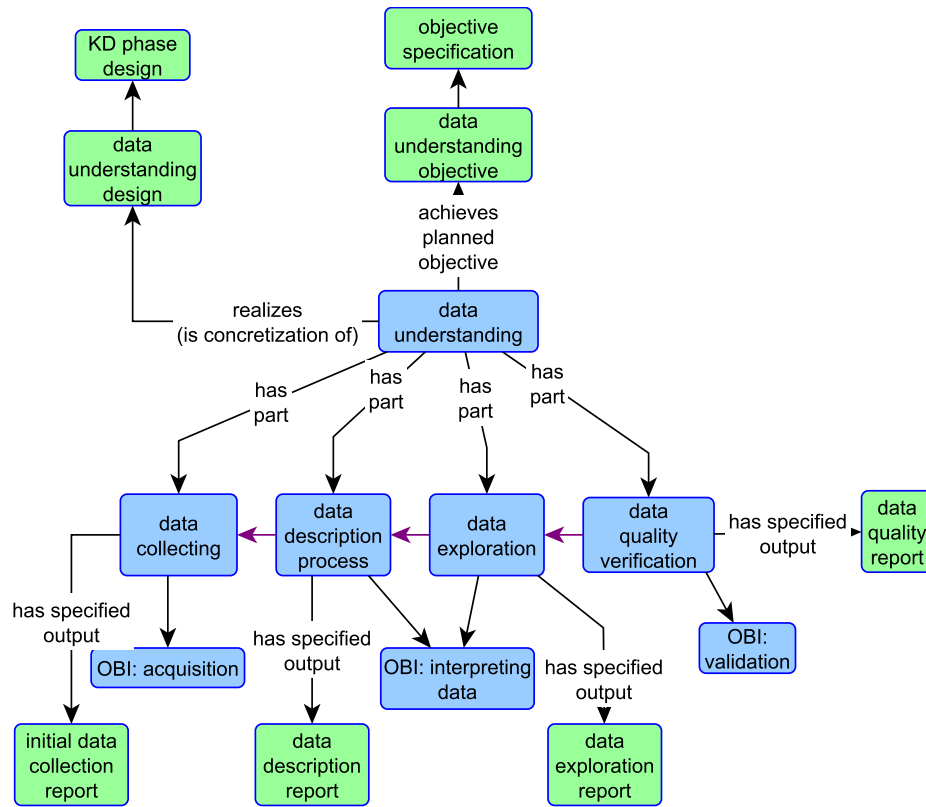
Figure 7.8: The data understanding process in OntoDM-KDD.
