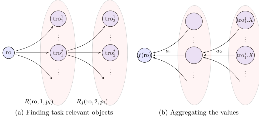
Figure 3: Two-step construction of a feature f in the internal nodes of a tree. In the example, the the considered foreign-key path p_i contains three tables. (a) Identification of all 1-related (i.e., R(ro, 1, p_i) ) and 2-related (i.e., R(ro, 2, p_i) ) task-relevant objects following p_i . (b) Aggregation of the value of the feature X , back to the target object.
