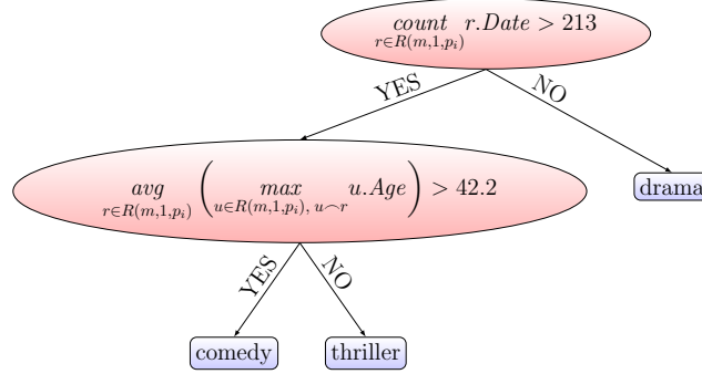
Figure 4: An example of tree built for the Movies dataset. In the root node, the reviews of the input movie m are counted (for technical reasons, we still need a predicate from the table Ratings , so the attribute Date was chosen). If the number of ratings is not greater than 213, the genre is predicted as drama . Otherwise, the average age of a user u who rated the movie m is computed (note that the age of a user is one single value and the aggregation function, max in this case, does not affect the result). If the average age is greater than 42.2, the predicted genre is comedy , otherwise it is thriller .
