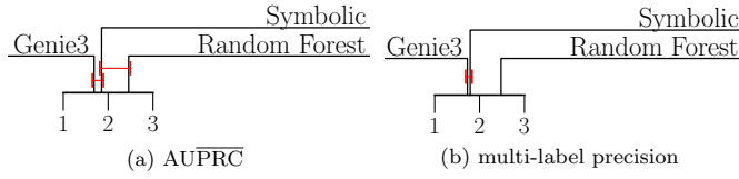
Fig. 7: The average rank diagrams of the proposed scores. Statistically significant differences are assessed by the Nemenyi post-hoc test. The quality of the rankings is measured in terms of AUPRC (a) and multi-label precision (b).
