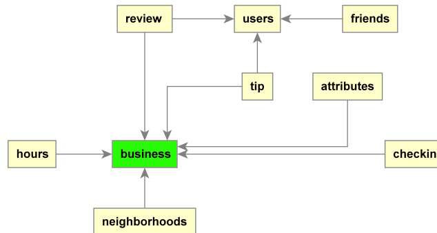
Figure 10: Schema of the dataset YELP, showing the tables and the foreign keys. The target table is emphasized in green.
