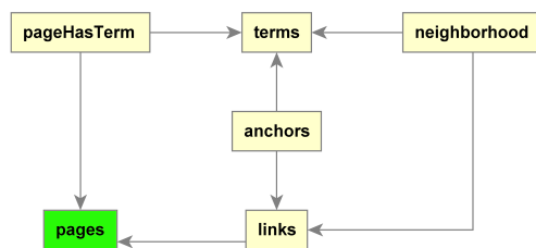
Figure 11: Schema of the dataset WEBKB, showing the tables and the foreign keys. The target table is emphasized in green.
