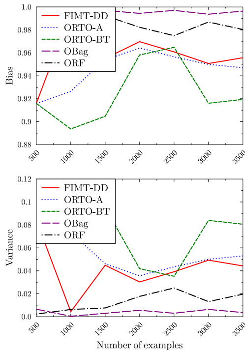
(a) Abalone
