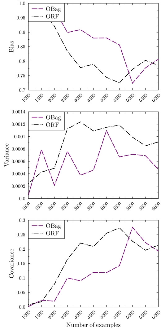
(a) Wind
