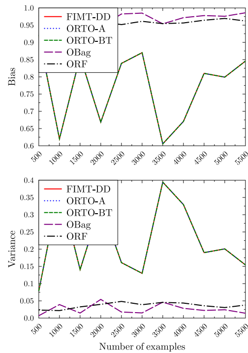
(a) Wind
