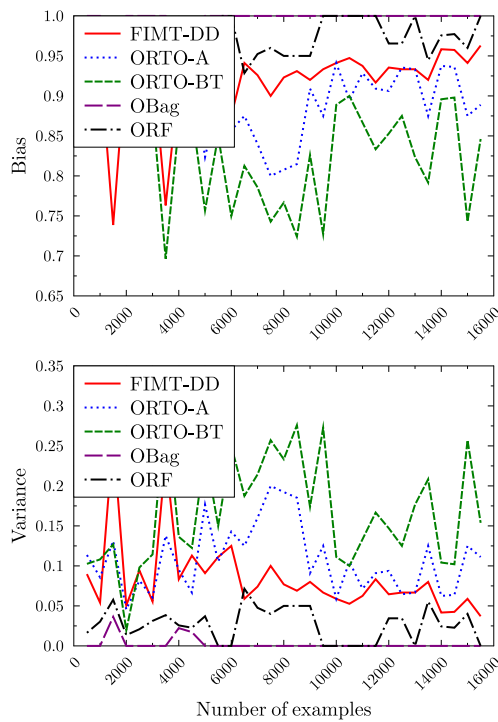
(c) Elevators
