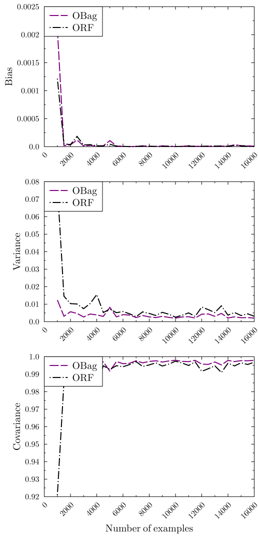
(a) Elevators
