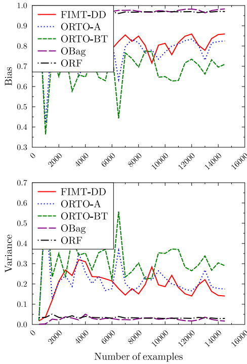
(c) Pol
